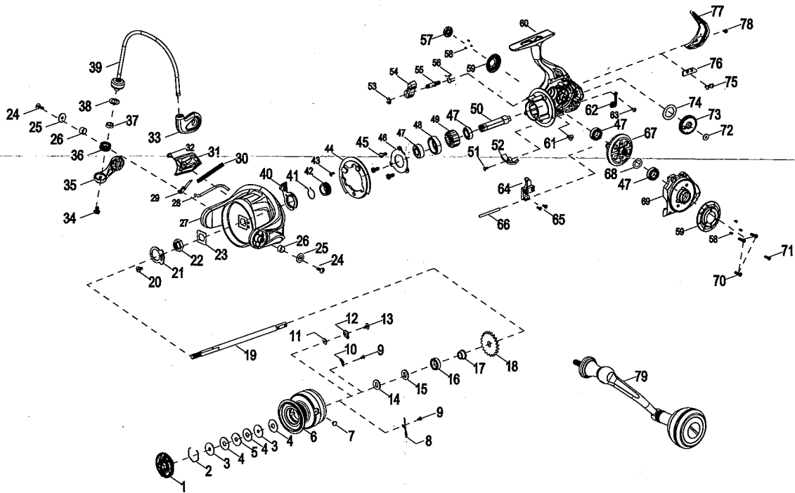
EXPLODED VIEW OF SGS8 8000-10000
